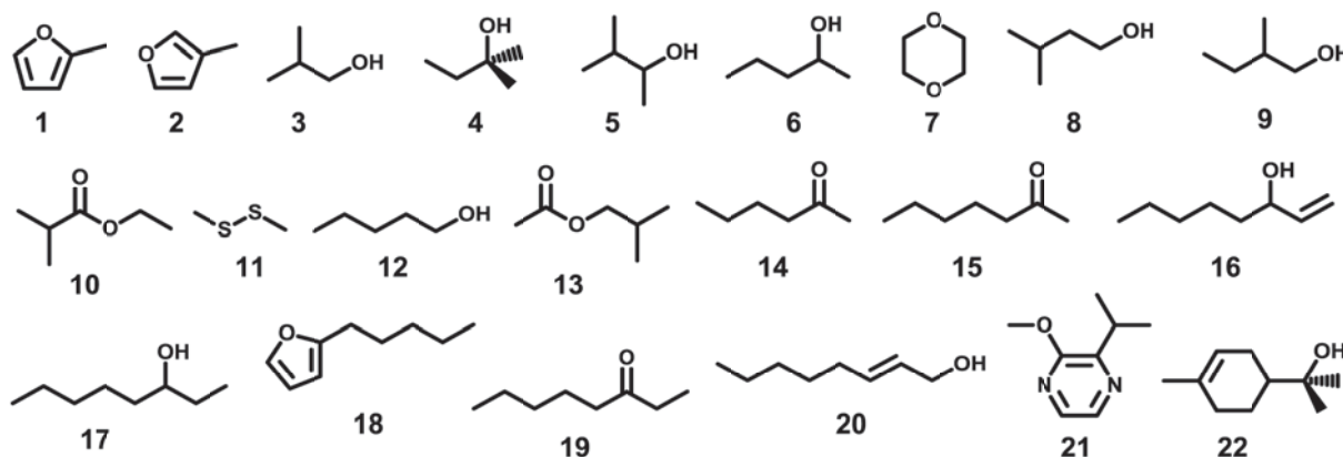
Fig. 1 Chemical Structures of the 22 MVOCs Measured in This Study
